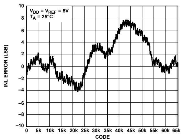
Figure 6. AD5667 INL, External Reference
